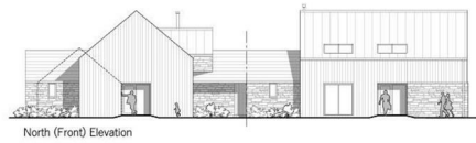
North (Front) Elevation
